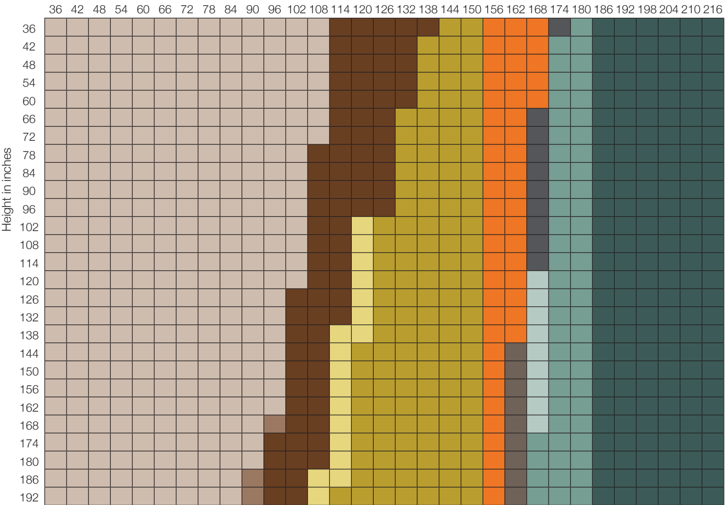
Motors and Fabric Weight Matrix Chart (for fabric weights ≤ 8.0 oz/sq yd)
