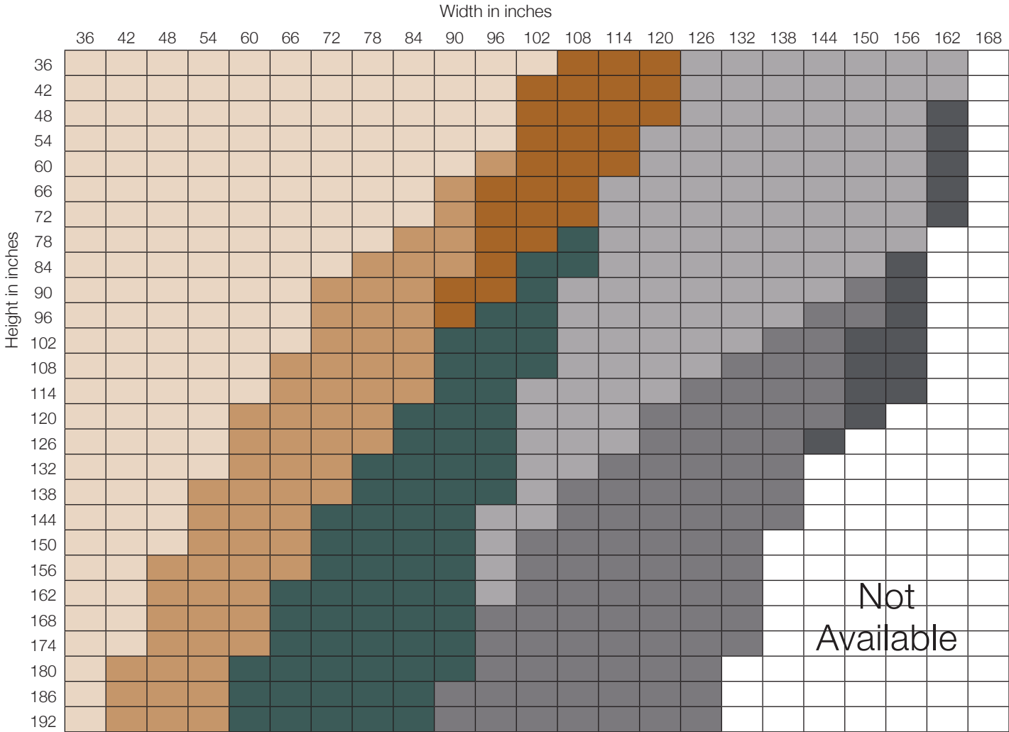
Motors and Fabric Weight Matrix Chart (for fabric weights ≥ 17.6 oz/sq yd)
