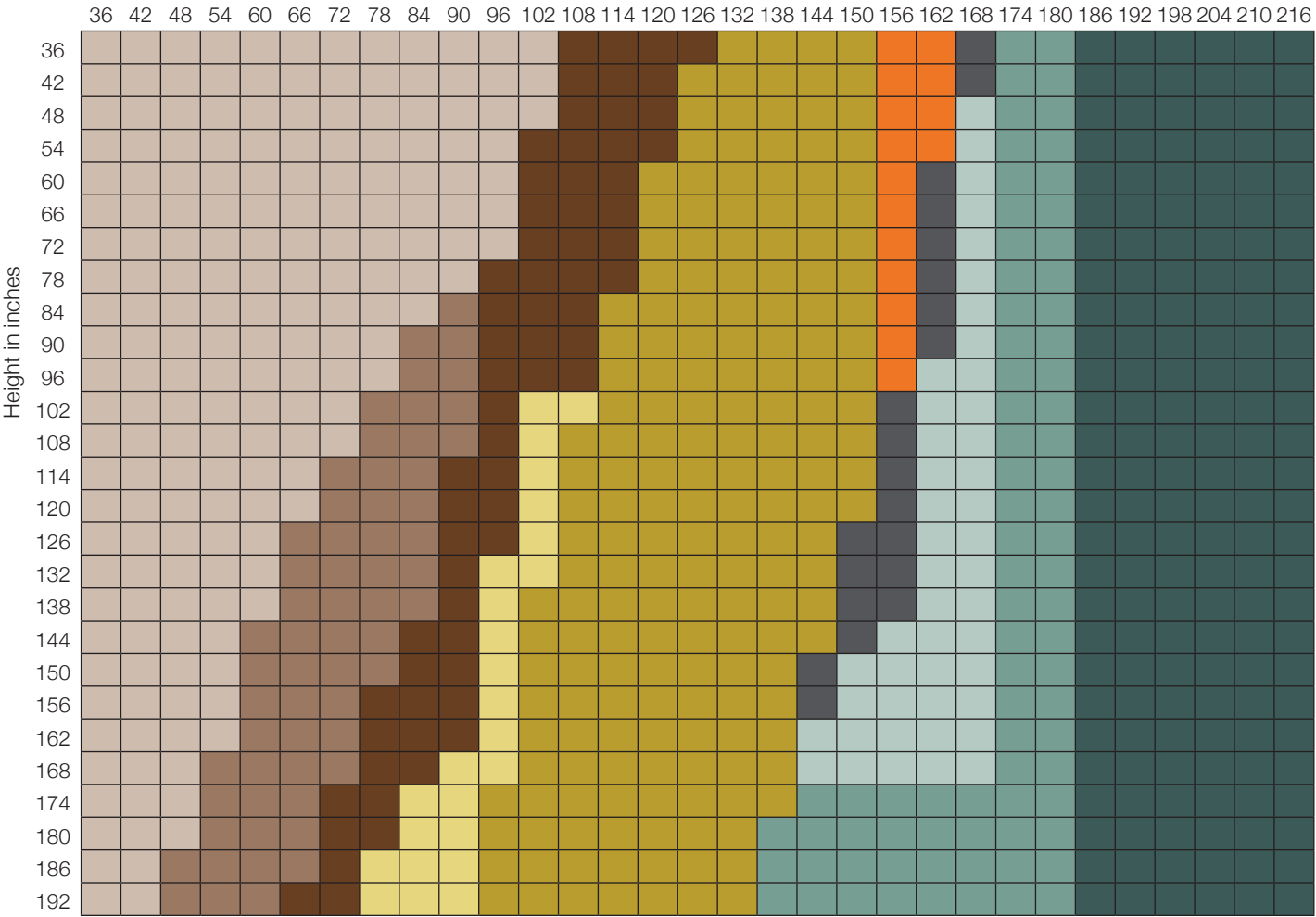
Motors and Fabric Weight Matrix Chart (for fabric weights 14.6 oz to 17.5 oz/sq yd)
