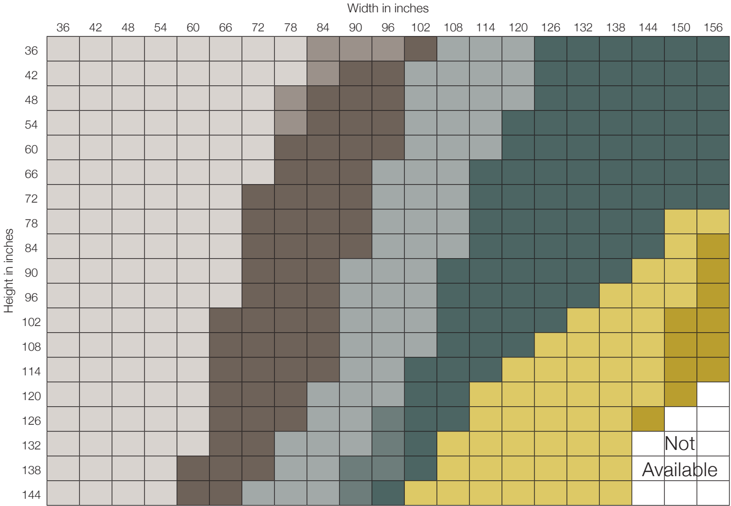
Clutch Tubes and Fabric Weight Matrix Chart (for fabric weights ≥ 17.6 oz/sq yd)
