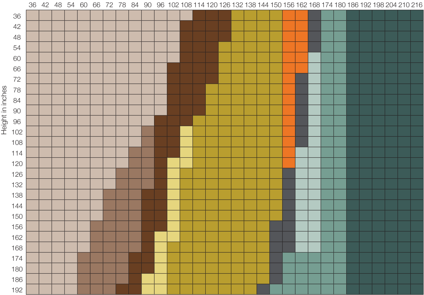
Motors and Fabric Weight Matrix Chart (for fabric weights 11.1 oz to 14.5 oz/sq yd)
