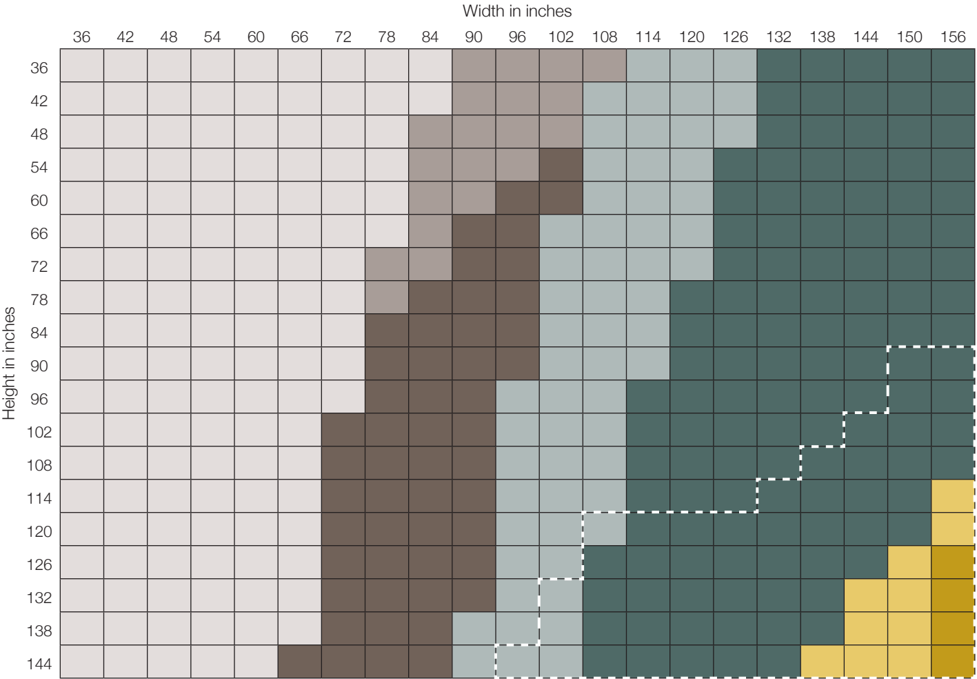
Clutch Tubes and Fabric Weight Matrix Chart (for fabric weights 11.1 oz to 14.5 oz/sq yd)
