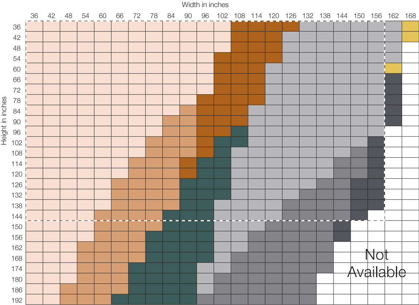
Motors and Fabric Weight Matrix Chart (for fabric weights 14.6 oz to 17.5 oz/sq yd)
