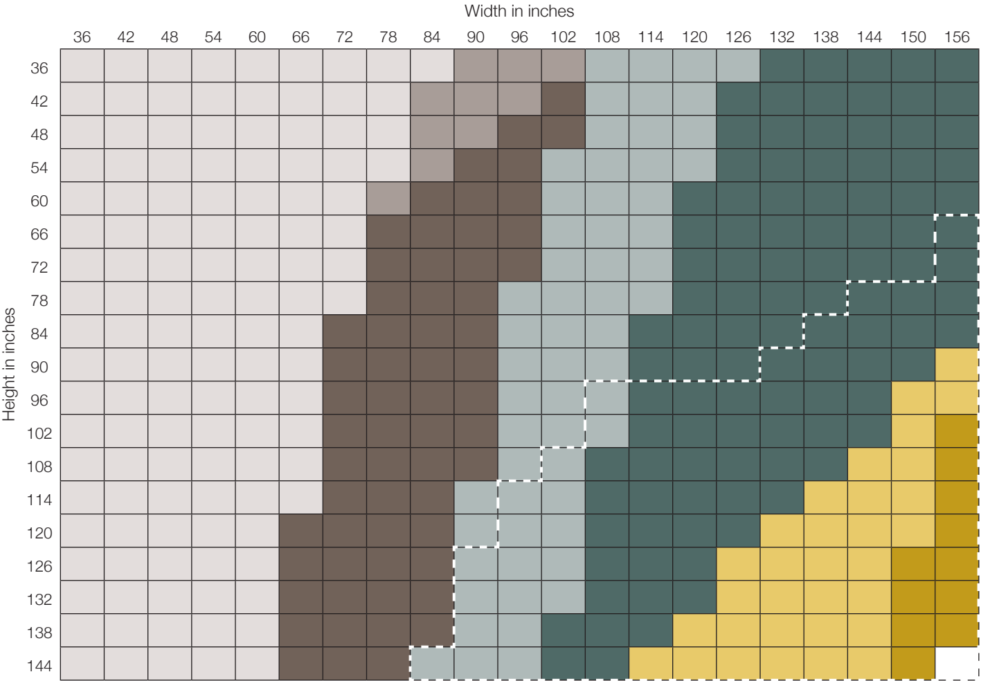
Clutch Tubes and Fabric Weight Matrix Chart (for fabric weights 14.6 oz to 17.5 oz/sq yd)
