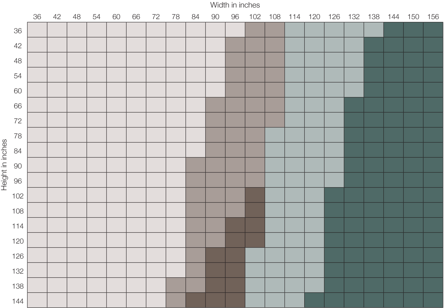
Clutch Tubes and Fabric Weight Matrix Chart (for fabric weights ≤ 8.0 oz/sq yd)
