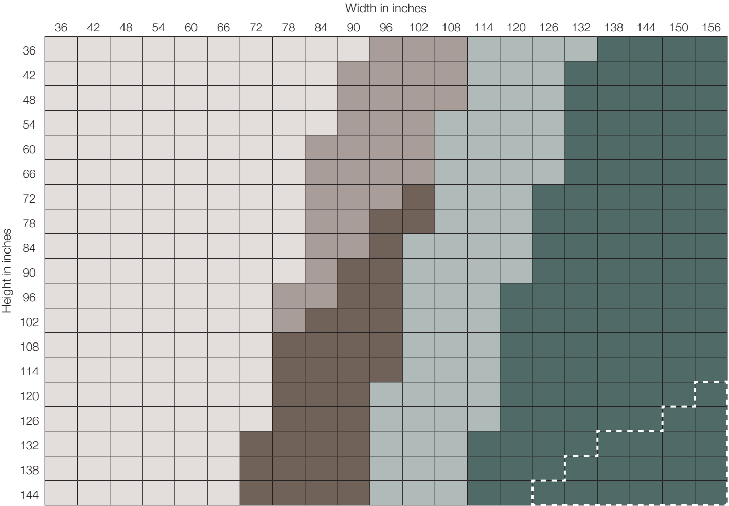
Clutch Tubes and Fabric Weight Matrix Chart (for fabric weights 8.1 oz to 11.0 oz/sq yd)
