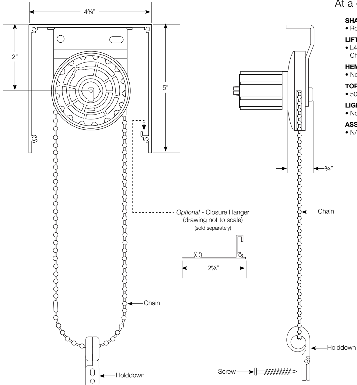
END VIEW (Shown without end cover)
