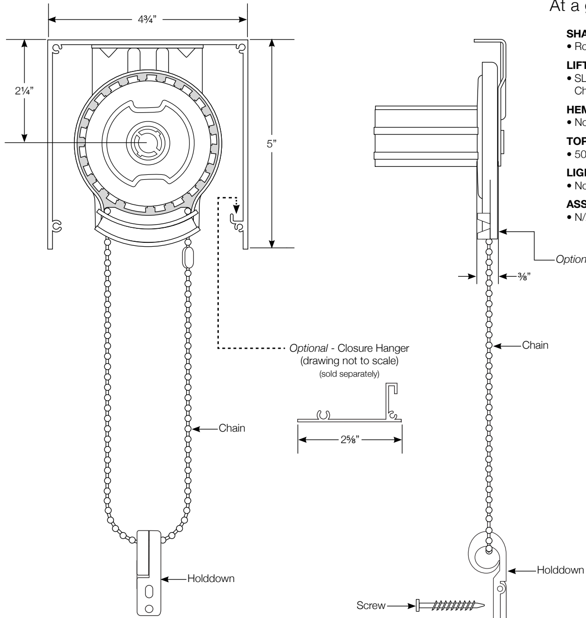
END VIEW (Shown without end cover)
