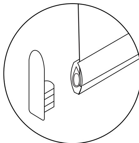
CLOSE-UP VIEW (Exposed Hem Bar and End Cap)
