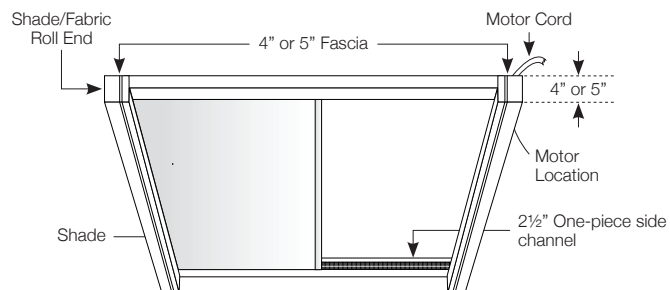
Side View of Skylight Slope:
