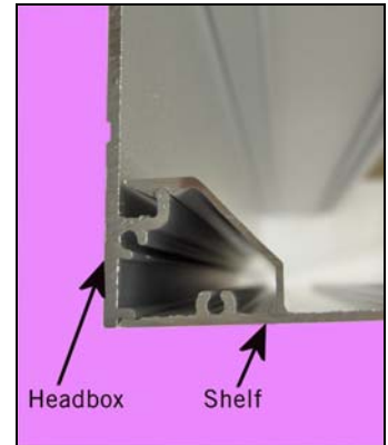
Figure 28 Shelf on Headbox
