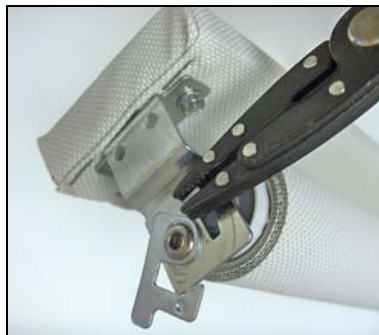
Figure 6 Placing Spring Pin in Spring Roller Bracket
