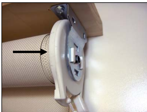
Figure 4 Clutch end aligned with bracket
